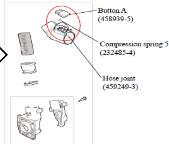
Dust nozzle assembly (127427-0)
